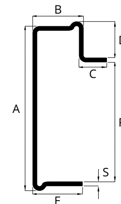
Longherina tipo Viberti / Viberti model floor frame profile
