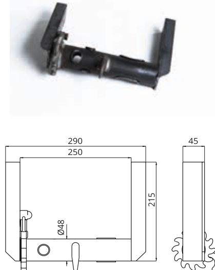
Verricello tendifune con tubino e asola Ø48 Winches with pipe and buttonhole Ø48
