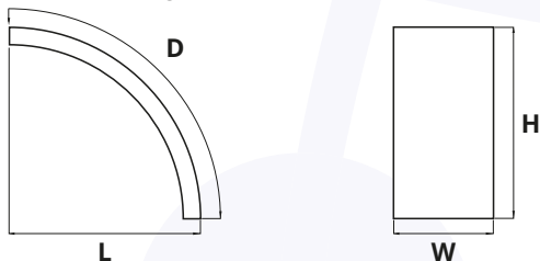
Curva Interflex inox gomma fiorettato Stainless steel rubber half-mudguard with texture and rubber edge
