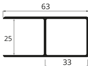
Testata in alluminio Aluminium lock profile, right
