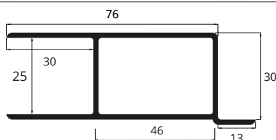
Montante VIP2 perno verticale con battuta Aluminium lock VIP2 with vertical pin and wing
