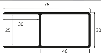
Montante VIP2 perno verticale senza battuta Aluminium lock VIP2 with vertical pin, without wing
